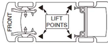
Unitized Body
